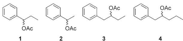
Scheme 1. Acetates 1–4 of secondary alcohols used in the kinetic resolution with the PLE isoenzymes.
