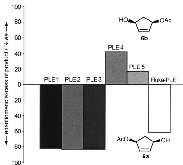
Figure 3. The enantiopreference of the recombinant PLE isoenzymes and of a commercial PLE isoenzyme mixture in the desymmetrization of 5 .
