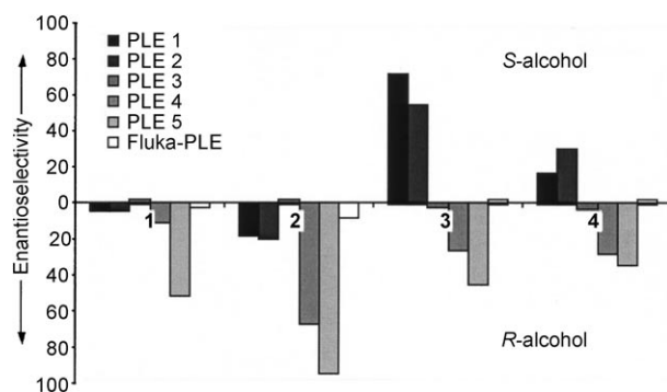
Figure 2. Enantioselectivity and enantiopreference of the recombinant PLE isoenzymes and commercial PLE isoenzyme mixture in the kinetic resolution of acetates 1–4 .
