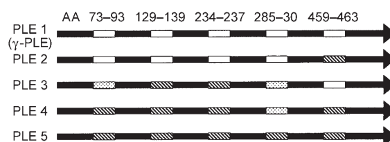
Figure 1. Differences between the isoenzymes are not randomly distributed, but occur in conserved areas. Black: homologous regions, white: variations in PLE1 ( \gamma -PLE), hashed: variations in PLE5, dotted: variations, which occur neither in PLE1 nor PLE5; AA = amino acid.
